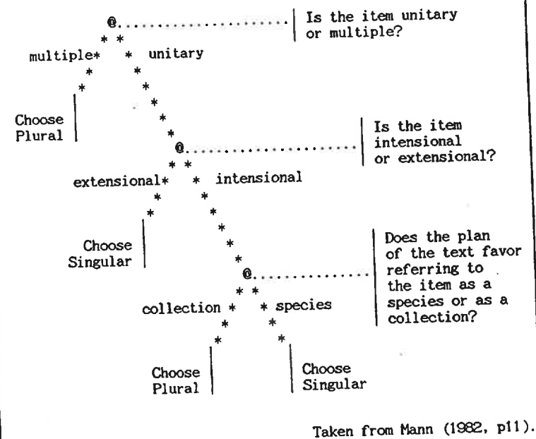
Figure 3: Chooser decision tree for the nominal group Number system
